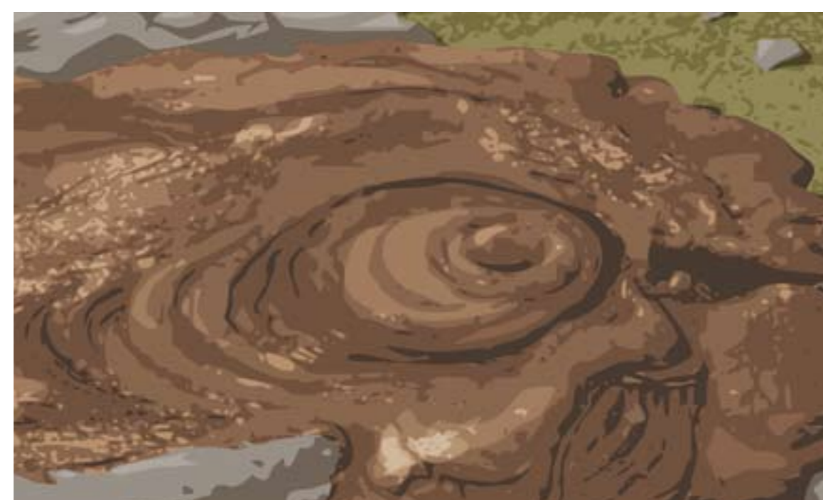
mud pot
