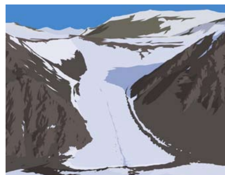
glacier
