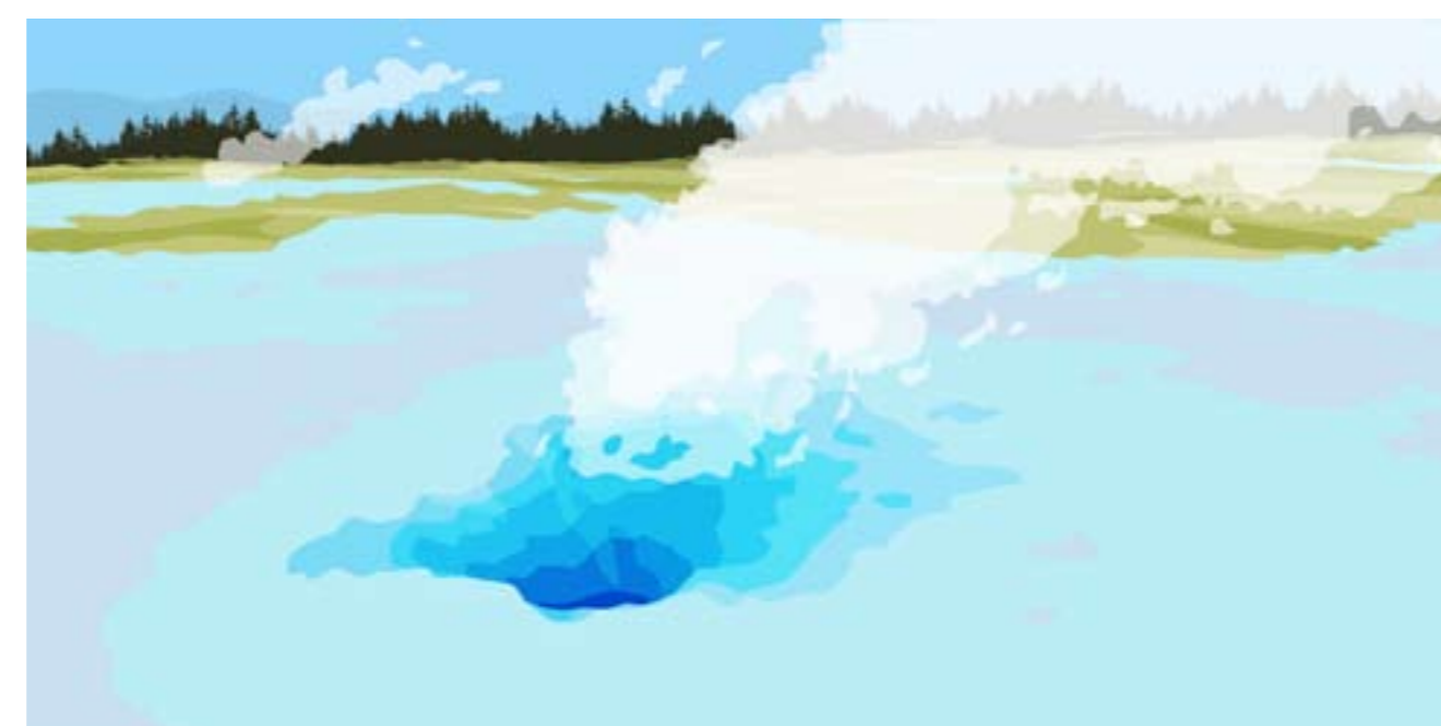
hot spring
