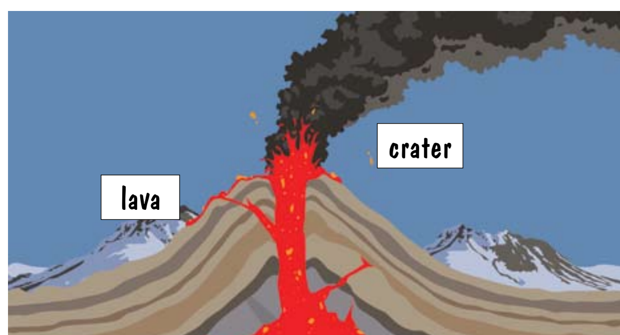
volcano
